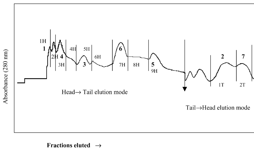
Fig. 2. HSCCC separation of the catechin crude extract from tea cultivar TRI 2025 Solvent system used Hex:EtOAc:MeOH:water 1:7:1:7. (+) Catechin 1, (+) CG 2, (–) EC 3, (–) EGC 4, (–) ECG 5, (–) ECGC 6, (–) ECGDG 7, 1H–9H (head–tail fractions), 1T–2T (tail–head fractions).
